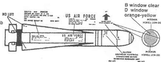
GBU-8 TV Guided Bomb
