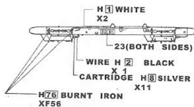
GBU-52
