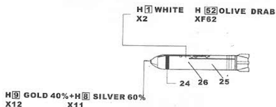
MK-20 ROCKEYE
